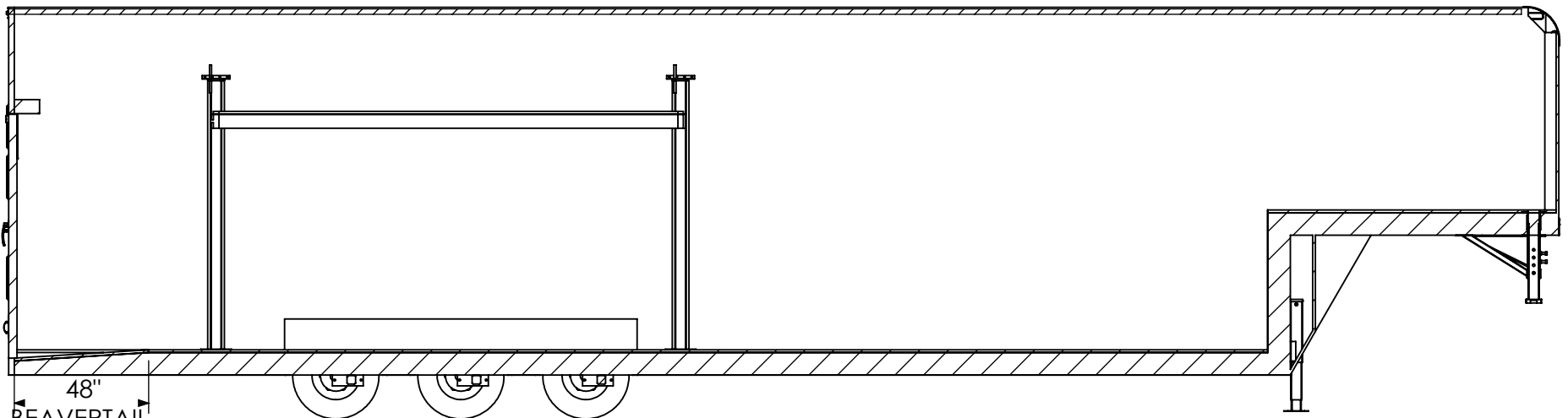
INTERIOR ROAD SIDE
