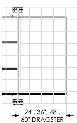
REAR EXTENSION
