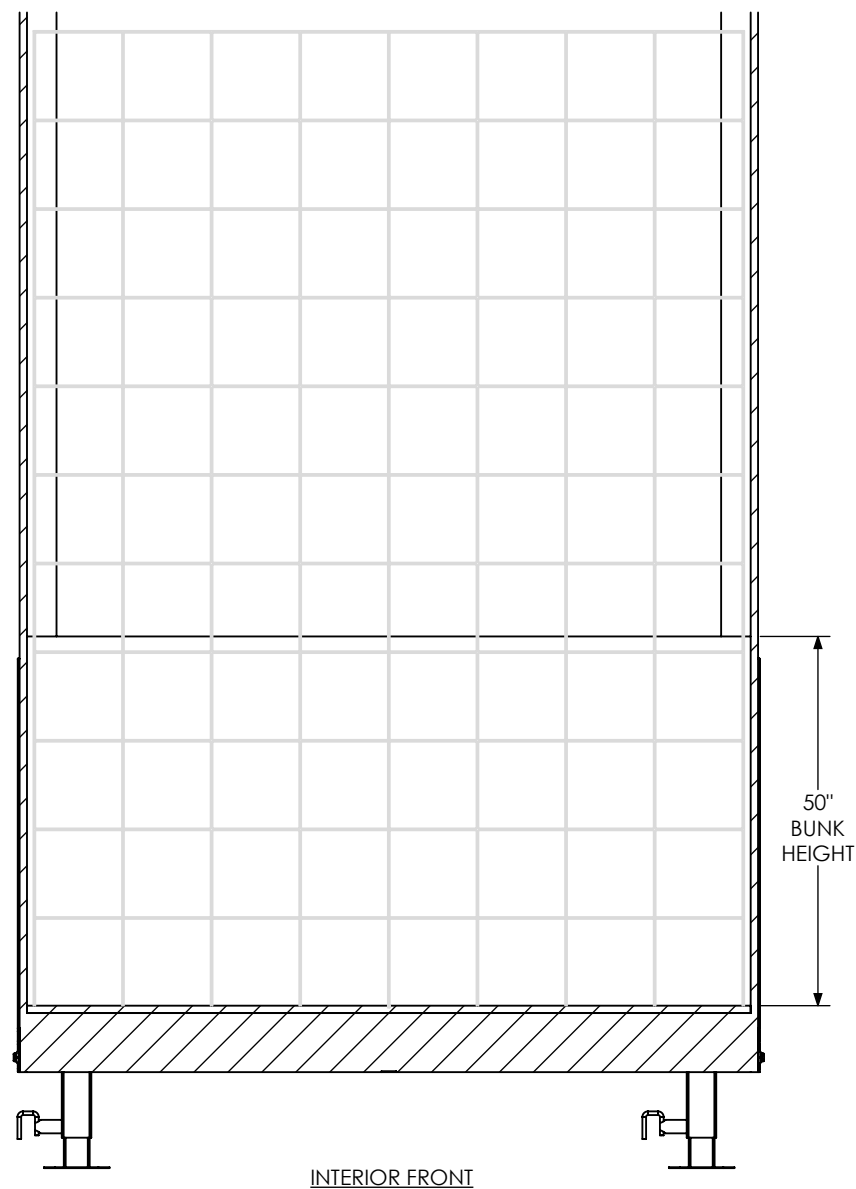
INTERIOR FRONT
